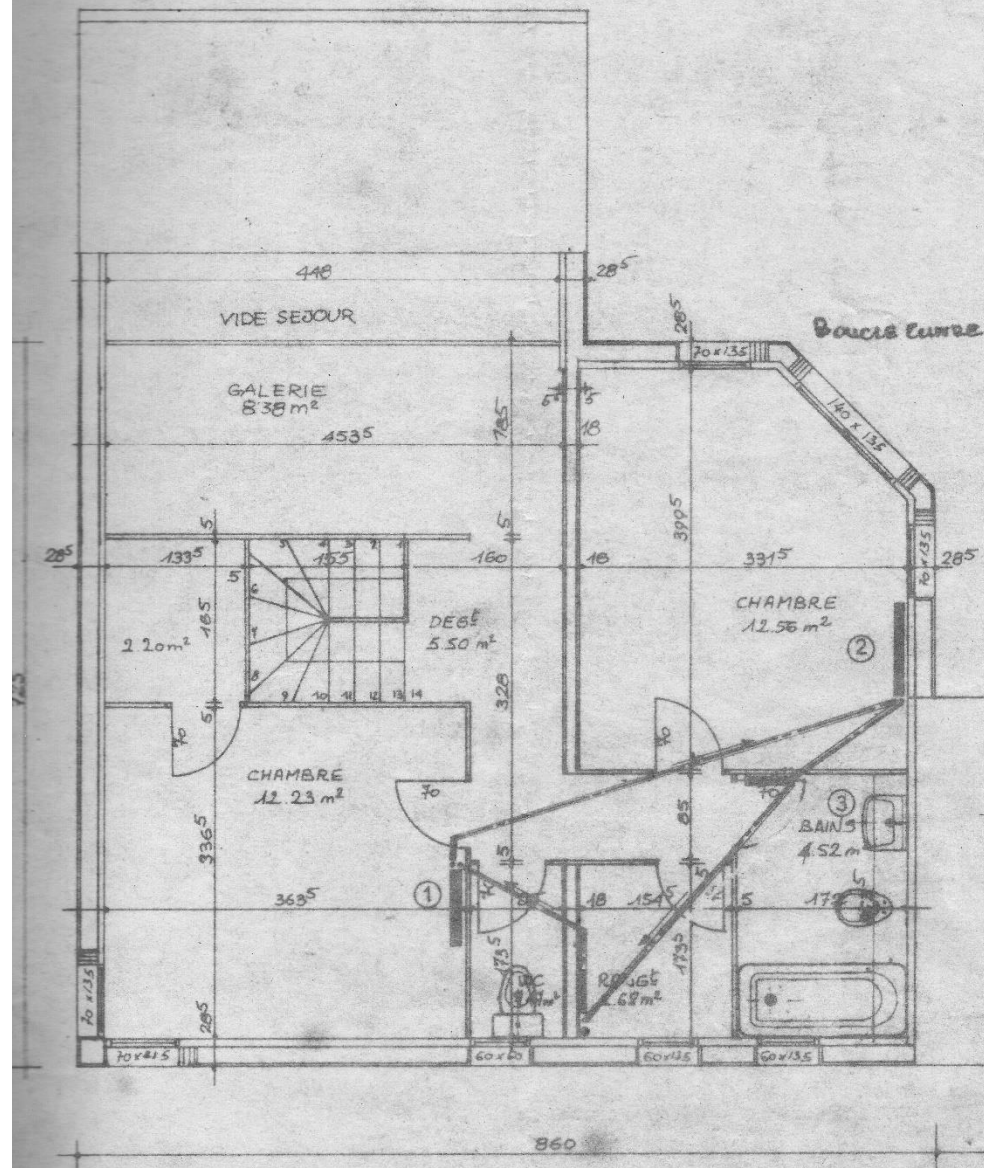
Courtine (type C) : plan chauffage (original de 1980)
